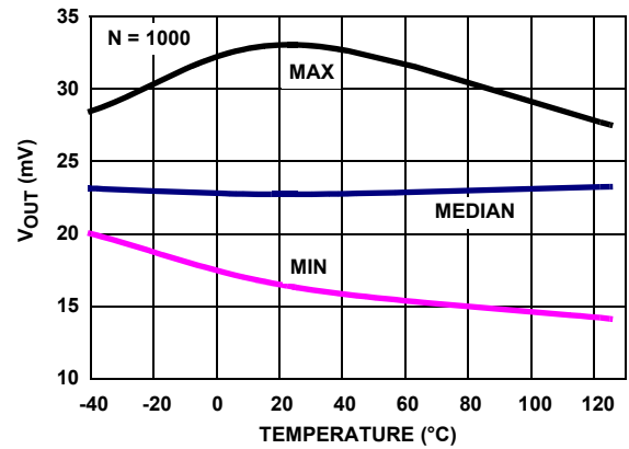
FIGURE 26. V_{OUT} LOW vs TEMPERATURE, V_+ = 5V , V_- = \pm 2.5V , R_L = 100k
