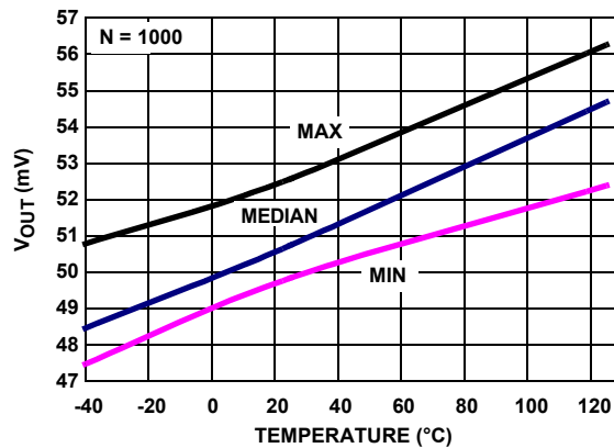
FIGURE 27. V_{OUT} LOW vs TEMPERATURE V_+ = 5V , V_- = \pm 2.5V , R_L = 10k
