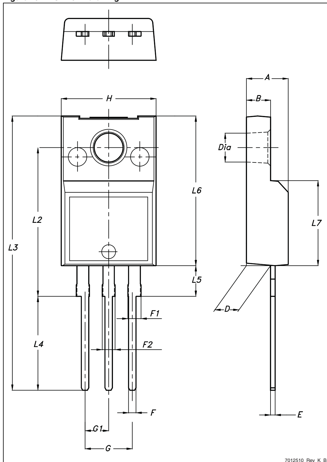
Figure 29. TO-220FP drawing
