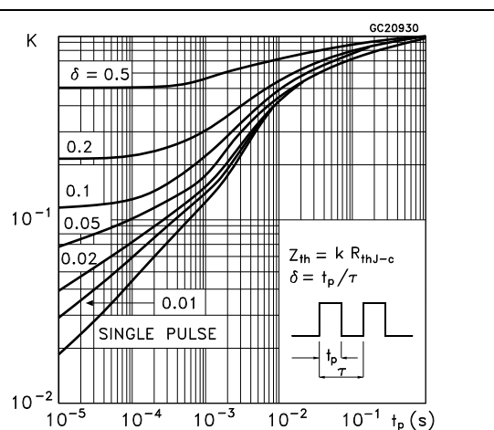
Figure 3. Thermal impedance for TO-220, D 2 PAK
