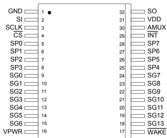
Figure 3. 33993 Pin Connections
