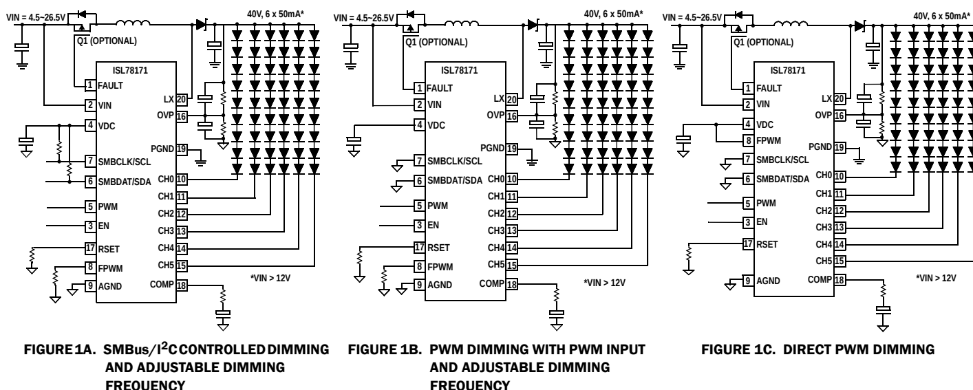
FIGURE 1. ISL78171 TYPICAL APPLICATION DIAGRAMS
