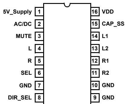
ISL54405 (16 LD TSSOP) TOP VIEW
