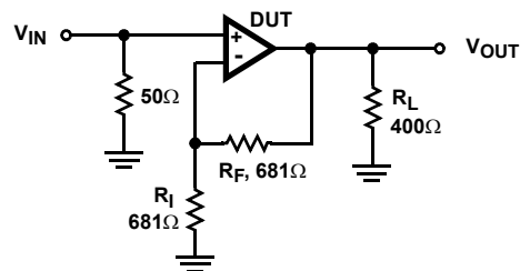
FIGURE 3. LARGE SIGNAL PULSE RESPONSE CIRCUIT
