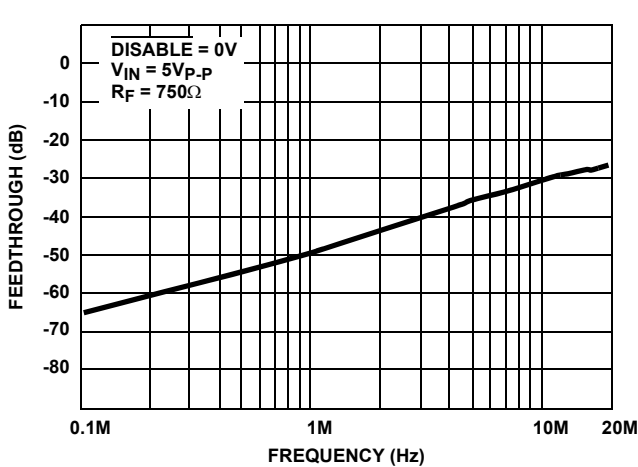
FIGURE 55. DISABLE FEEDTHROUGH vs FREQUENCY
