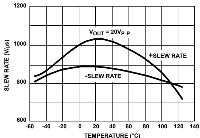
FIGURE 38. SLEW RATE vs TEMPERATURE (AVERAGE OF 30 UNITS FROM 3 LOTS)
