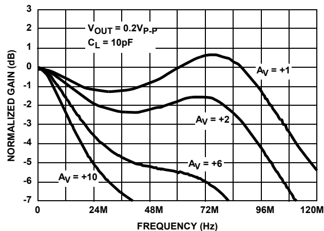
FIGURE 20. NON-INVERTING GAIN vs FREQUENCY
