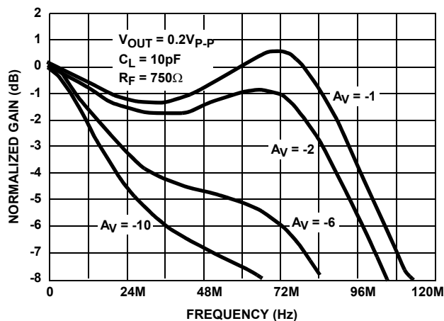
FIGURE 21. INVERTING FREQUENCY RESPONSE
