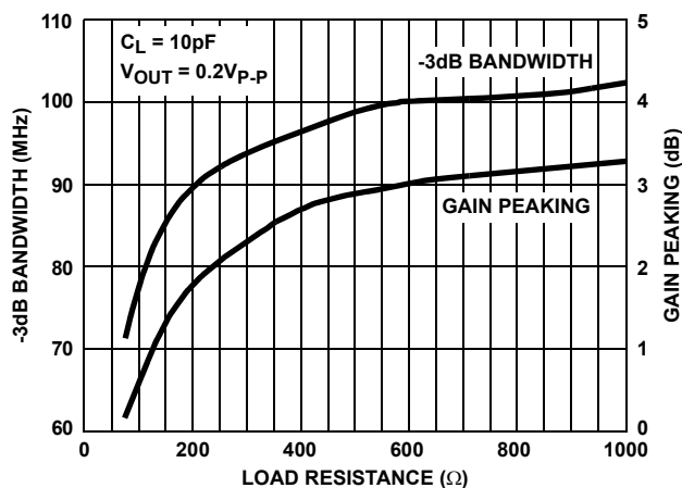
FIGURE 23. BANDWIDTH AND GAIN PEAKING vs LOAD RESISTANCE
