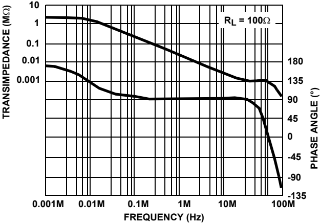
FIGURE 56. TRANSIMPEDANCE vs FREQUENCY
