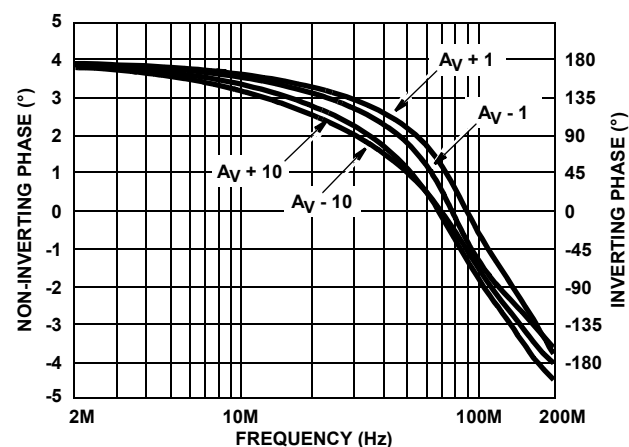
FIGURE 41. PHASE RESPONSE AS A FUNCTION OF FREQUENCY
