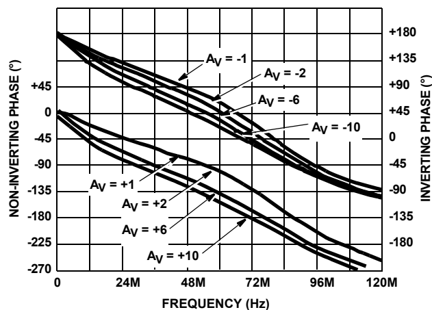
FIGURE 22. PHASE vs FREQUENCY
