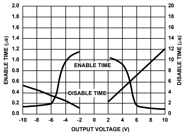
FIGURE 19. ENABLE/DISABLE TIME vs OUTPUT VOLTAGE (AVERAGE OF 9 UNITS FROM 3 LOTS)
