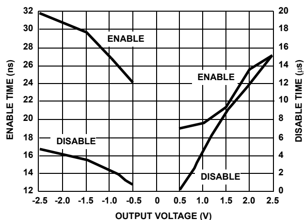
FIGURE 54. ENABLE/DISABLE TIME vs OUTPUT VOLTAGE
