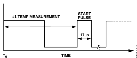
Figure 27. Daisy-Chain Temperature Measurement and Start Pulse Output from First TMP05/TMP06
