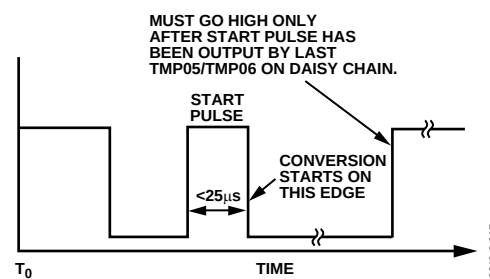
Figure 26. Start Pulse at CONV/IN Pin of First TMP05/TMP06 Device on Daisy Chain
