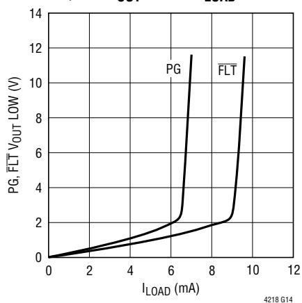
PG, \overline{\text{FLT}} V_{\text{OUT Low}} vs I_{\text{LOAD}}
