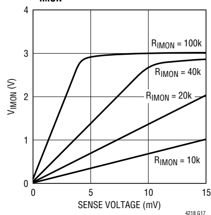
V_{\text{IMON}} vs Sense
