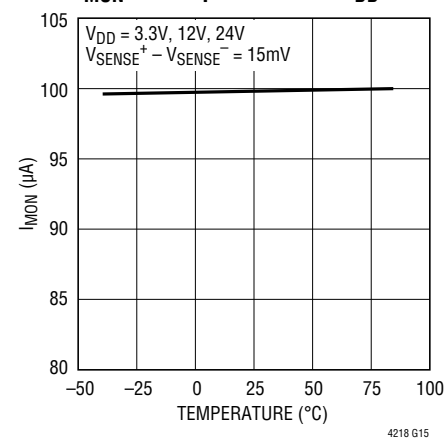
I_{\text{MON}} vs Temperature and V_{DD}
