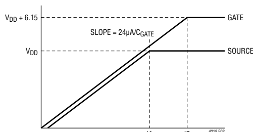
Figure 2. Supply Turn-On
