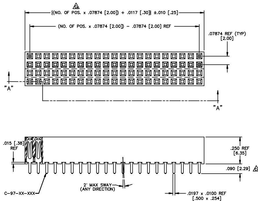
SECT. "A-A"
