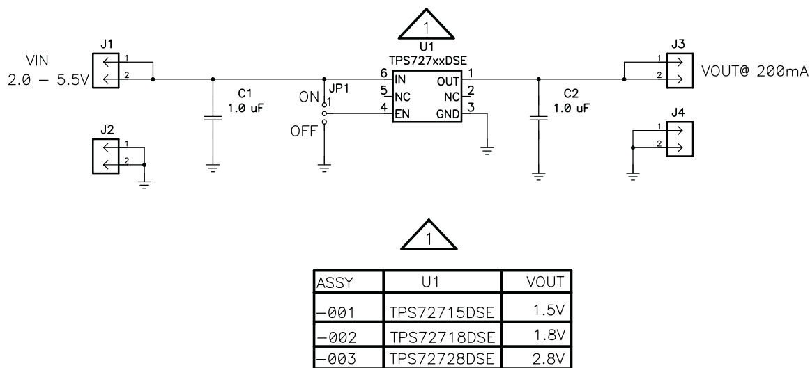
Figure 5. TPS727xxDSEEM-406 Schematic
