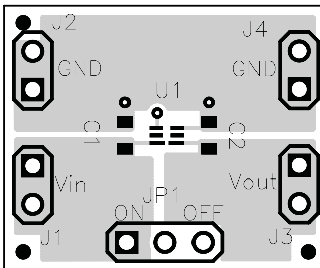
Figure 1. Top Layer Assembly
