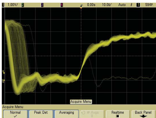
Figure 5. 256 levels of display intensity gradation show characteristics of jitter, noise, and signal anomalies.
