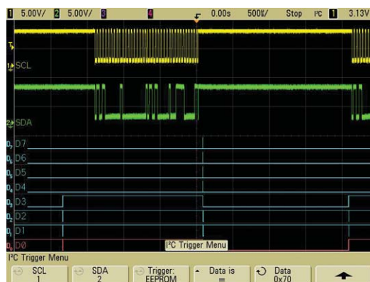
Figure 11. Trigger on address and/or data patterns within an I 2 C frame.
