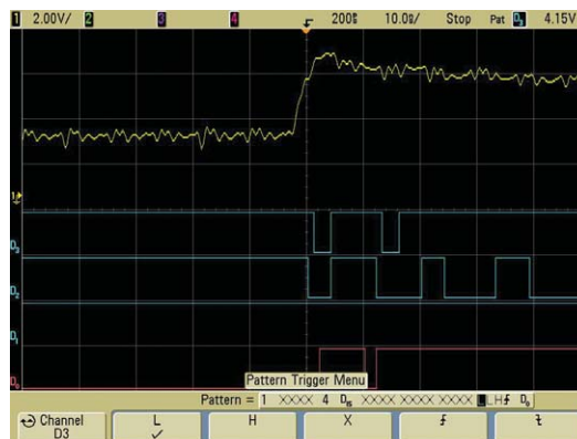
Figure 10. MSOs provide advanced pattern triggering across all scope AND logic channels for quick isolation of critical events.
