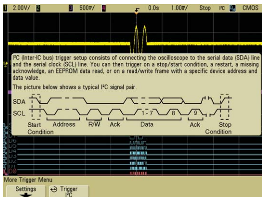
Figure 12. Press and hold any key for built-in Help, such as this description of the I²C bus triggering.
