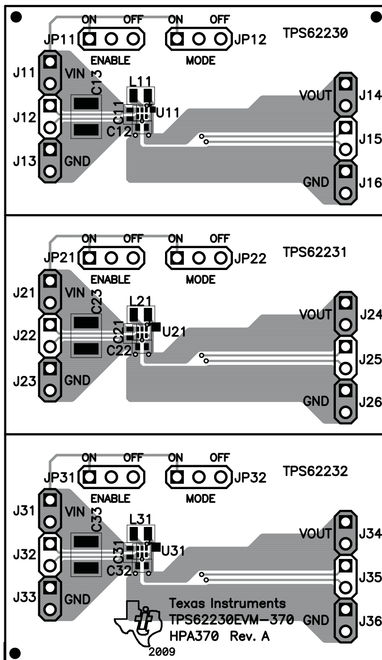
Figure 1. Assembly Layer
