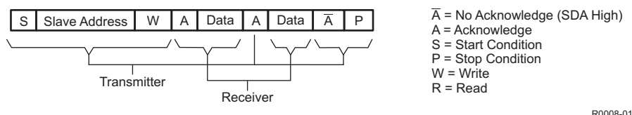
Figure 42. I²C Read Cycle
