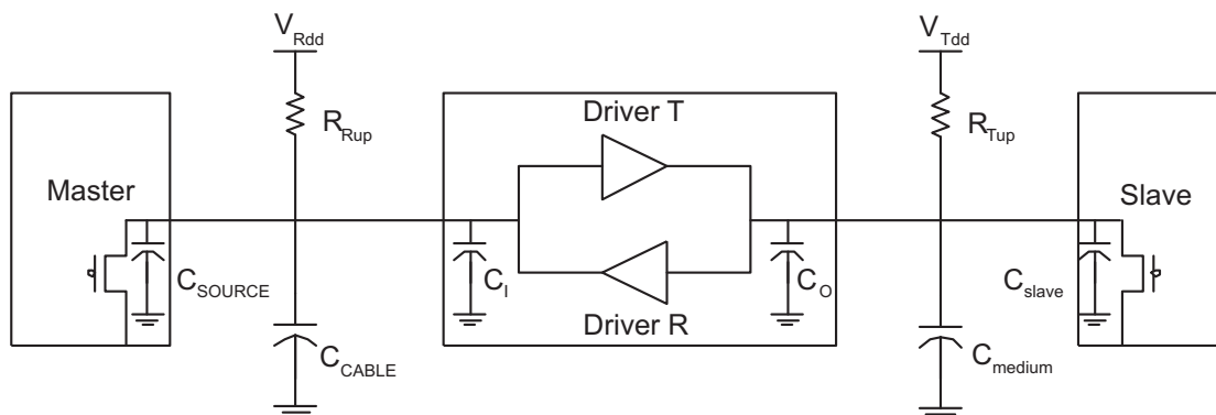
Figure 30. Typical Application
