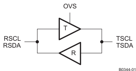
Figure 28. I 2 C Drivers in the TMD5361 (R Side Is the HDMI Source Side, T Side Is the HDMI Sink Side)
