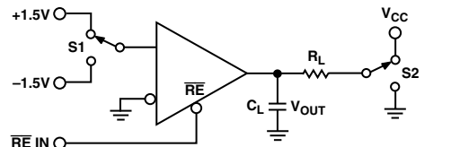
Figure 6. Receiver Enable/Disable Test Circuit
