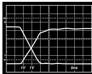
Figure 22. Unloaded Driver Differential Outputs
