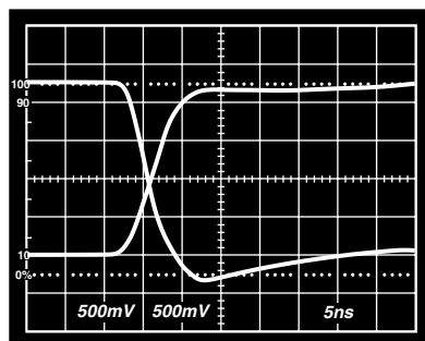
Figure 23. Loaded Driver Differential Outputs
