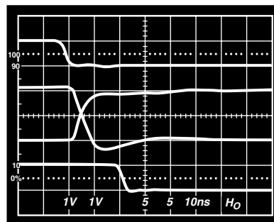
Figure 25. Driver/Receiver Propagation Delays High to Low
