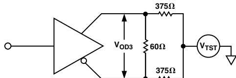
Figure 2. Driver Voltage Measurement Test Circuit 2
