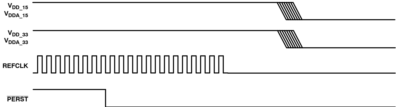
Figure 3–3. Power-Down Sequence
