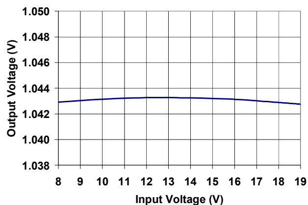
Figure 10: Line Regulation at I_{OUT} = 15A
