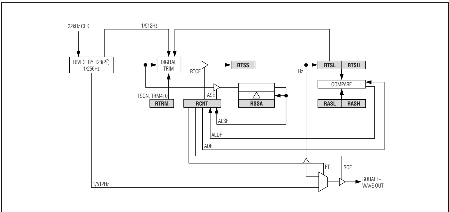
Figure 14-1. RTC Functional Block Diagram
