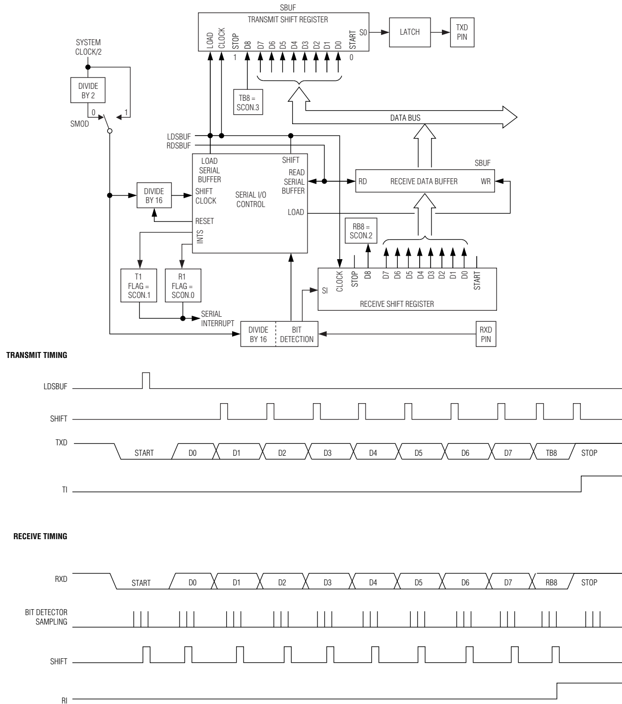
Figure 10-3. UART Mode 2
