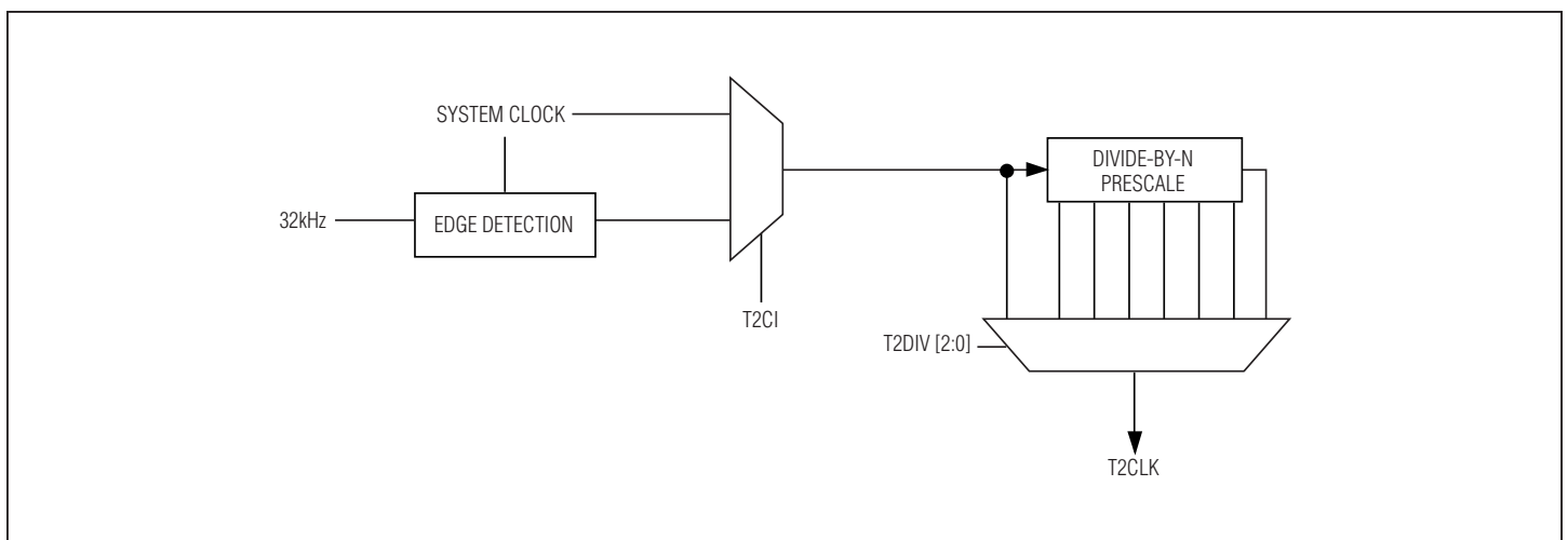
Figure 9-3. Timer 2 Clock
