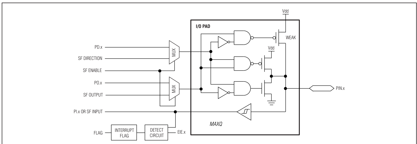
Figure 6-4. Type D Port Pin Schematic
