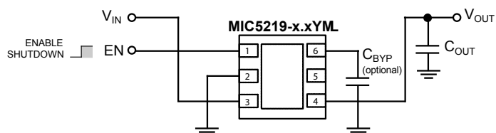
Ultra-Low-Noise Regulator (Fixed)
