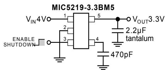
3.3V Ultra-Low-Noise Regulator
