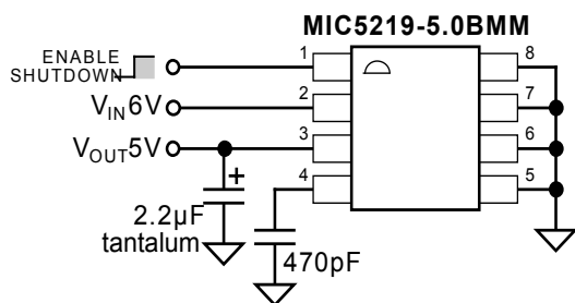
5V Ultra-Low-Noise Regulator
