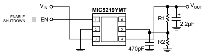
Ultra-Low-Noise Regulator (Adjustable)
