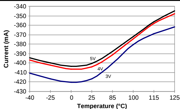
SHORT CIRCUIT CURRENT VS TEMPERATURE
