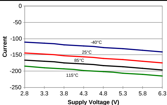
OUTPUT CURRENT VS SUPPLY VOLTAGE
