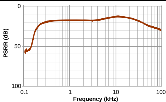
PSRR VS FREQUENCY IN DROPOUT
