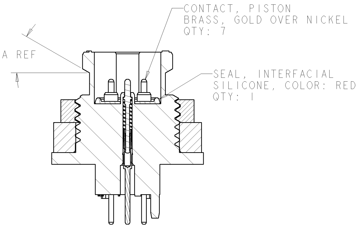
SECTION X-X
