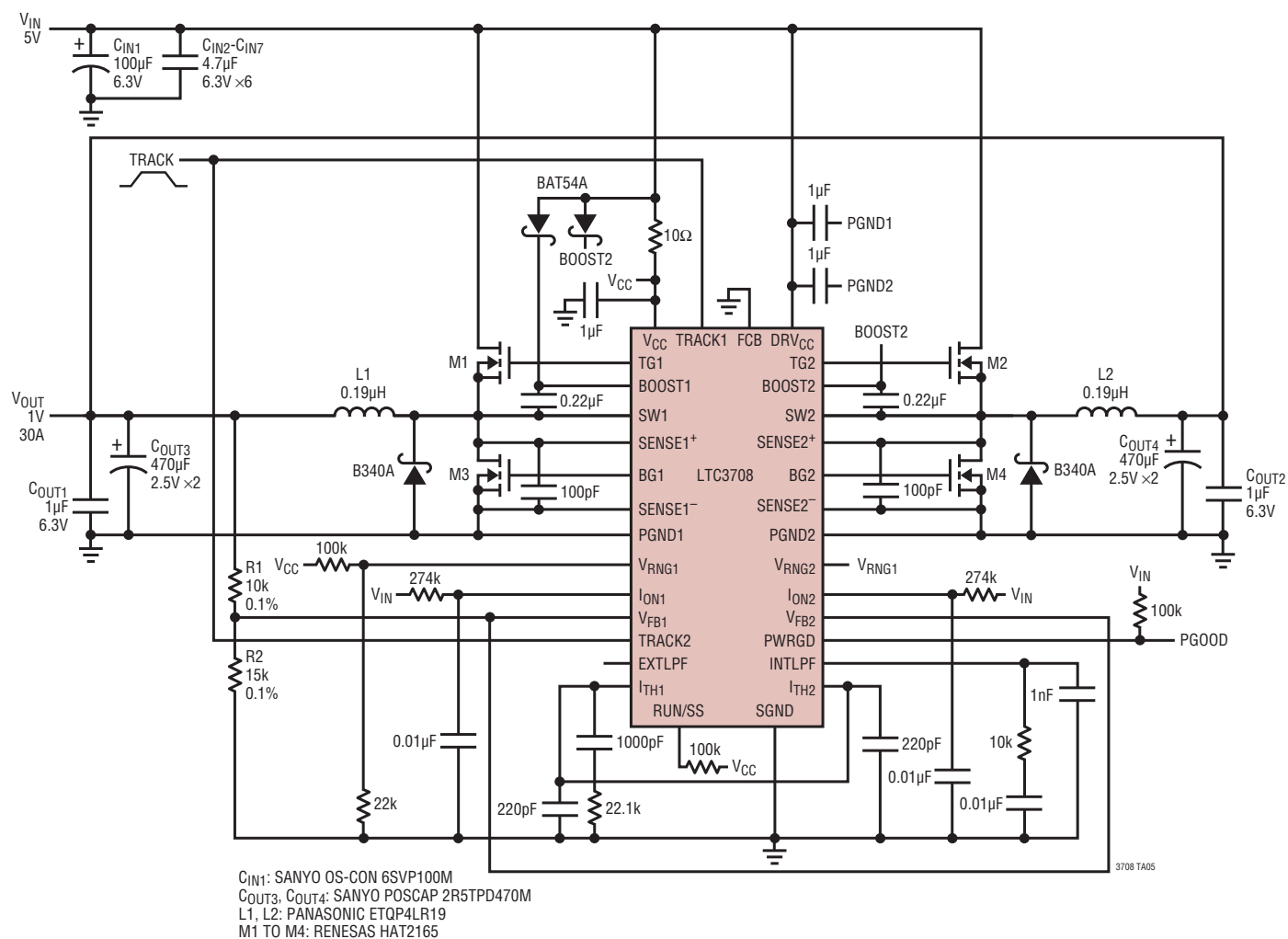
Dual-Phase, 30A Power Supply with 10mV Output Ripple
