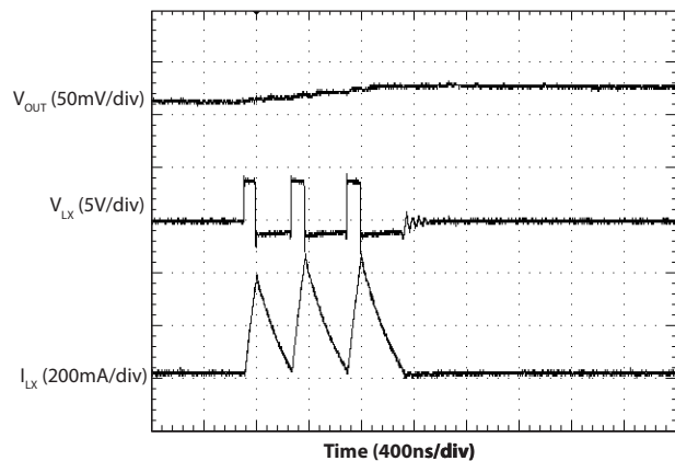
Light Load Switching — V_{OUT} = 2.8V
