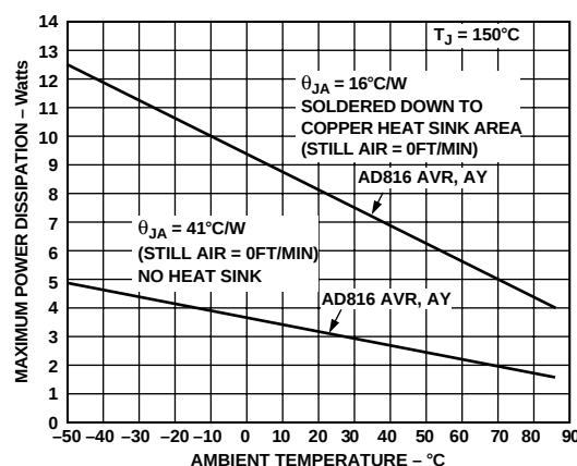
Figure 1. Plot of Maximum Power Dissipation vs. Temperature (Copper Heat Sink Area = 2\text{ in.}^2 )
