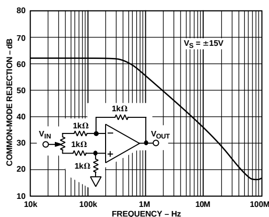
Figure 7. Driver Common-Mode Rejection vs. Frequency
