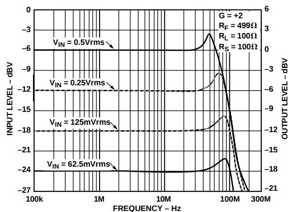
Figure 17. Driver Small and Large Signal Frequency Response, G = +2
