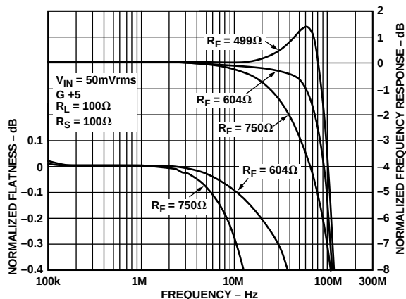
Figure 18. Driver Frequency Response and Flatness, G = +5
