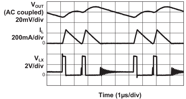
Light Load Switching Waveform (LL Mode; V_{IN} = 4.2V ; V_{OUT} = 0.6V ; R_L = 10\Omega ; C_{OUT} = 4.7\mu F ; L = 2.2\mu H )
