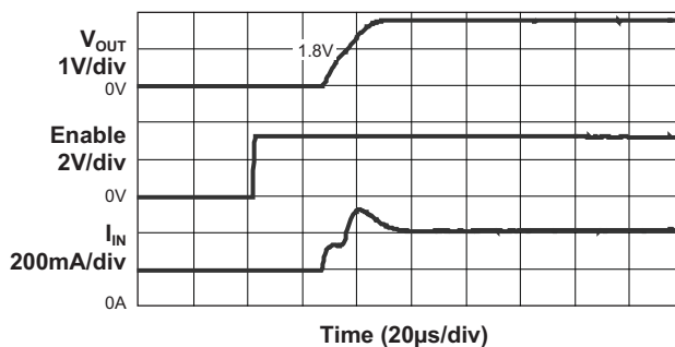
Enable Soft Start ( V_{IN} = 3.6V ; V_{OUT} = 1.8V ; R_L = 3.9\Omega ; C_{OUT} = 4.7\mu F ; L = 2.2\mu H )
