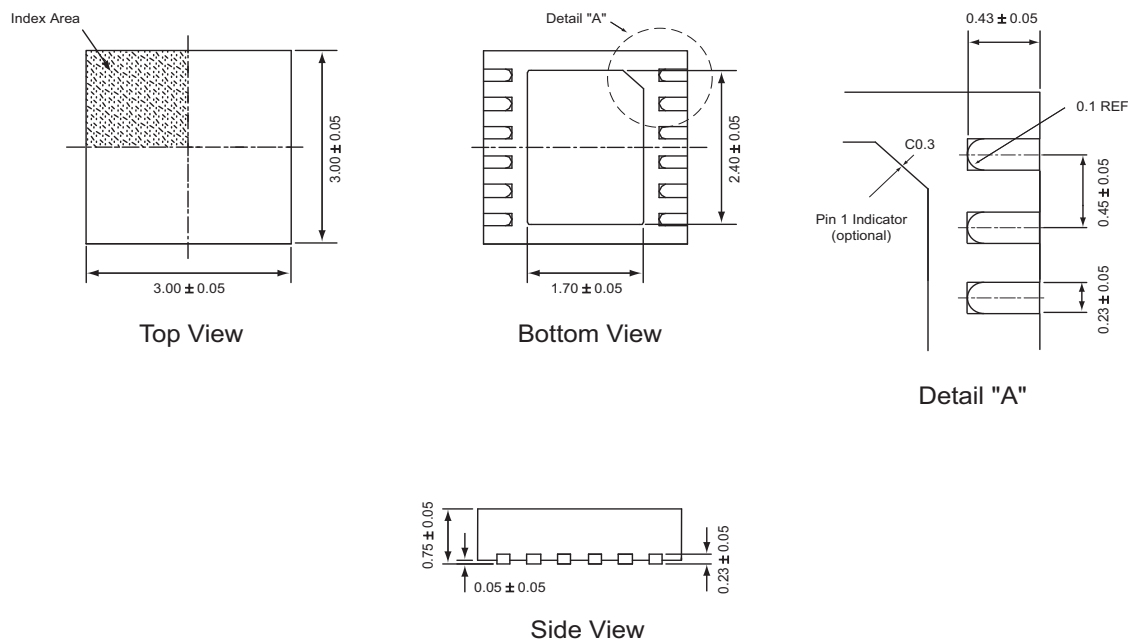
TDFN33-12
