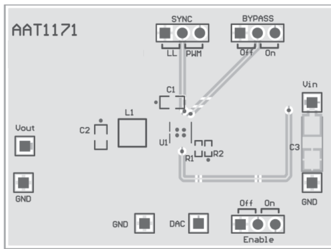
Figure 5: AAT1171 Evaluation Board Bottom Side Layout.
