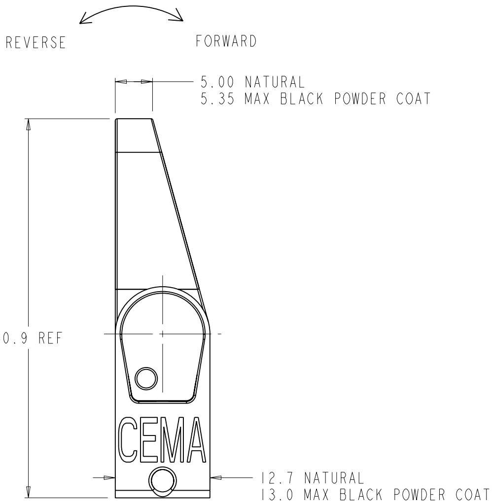
TYPE B (SHOWN DIMENSIONED)
