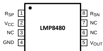
Figure 3. Top View
