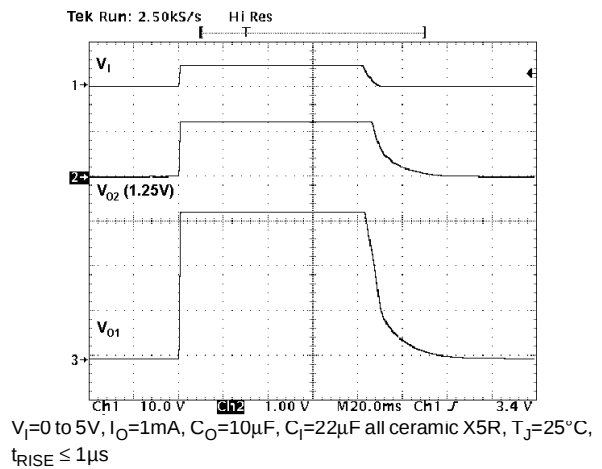
Figure 28 : Start-Up Transient
