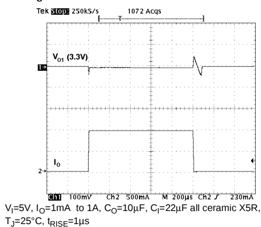
Figure 24 : Change of V_O with Step Load Change
