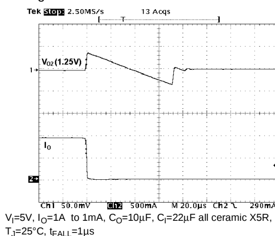
Figure 22 : Change of V_O with Step Load Change
