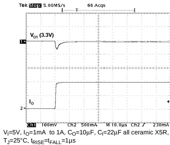
Figure 26 : Change of V_O with Step Load Change
