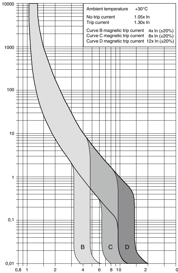
Figure 1 Trip curves
