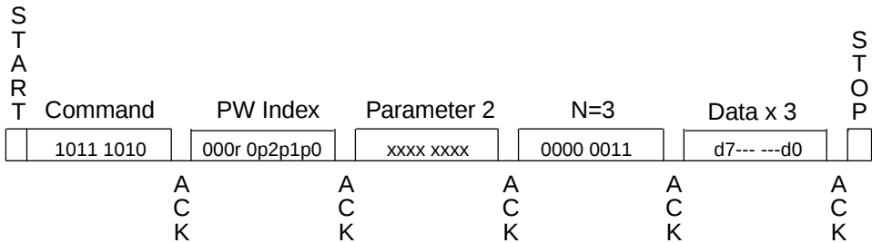
Figure 7-15. Verify Password
