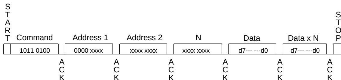
Figure 7-9. System Write
