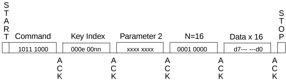
Figure 7-13. Verify Crypto
