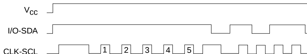
Figure 7-1. Start-up Sequence
