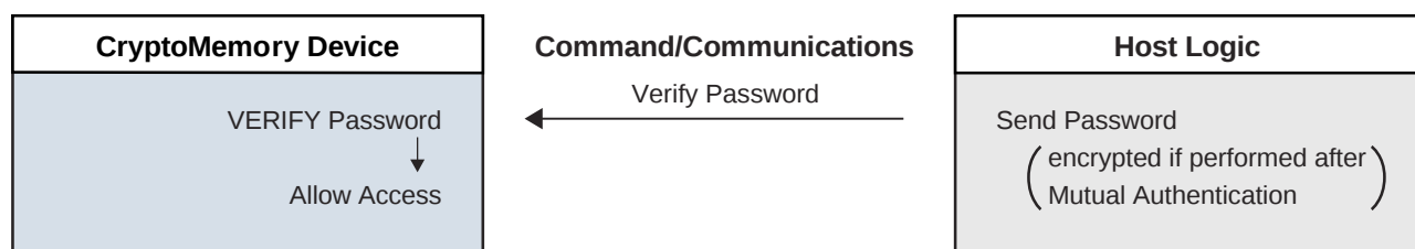
Figure 5-1. Password Verification
