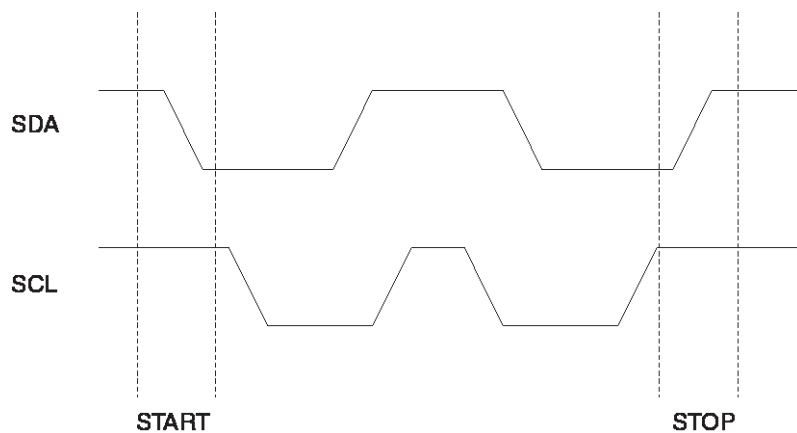
Figure 11-4. Start and Stop Definition
