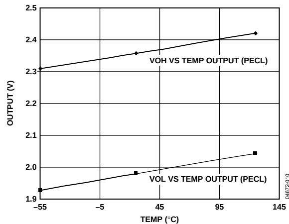
Figure 10. ADCMP582 Output Voltage vs. Temperature
