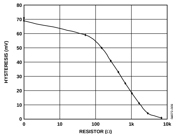
Figure 9. Hysteresis vs. R_{HYS} Control Resistor
