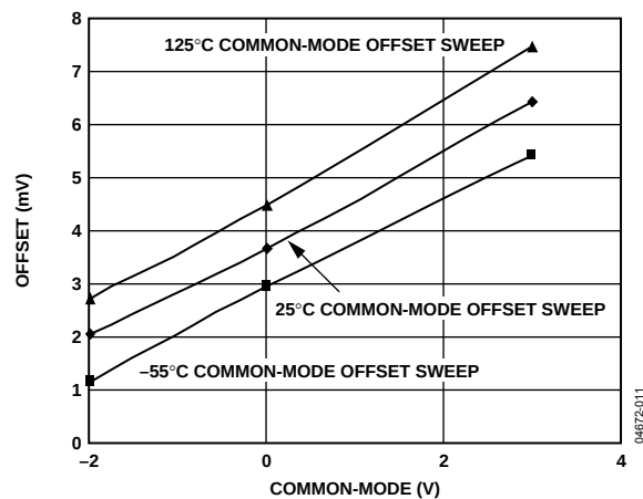
Figure 11. A Typical VOS vs. Common-Mode Voltage
