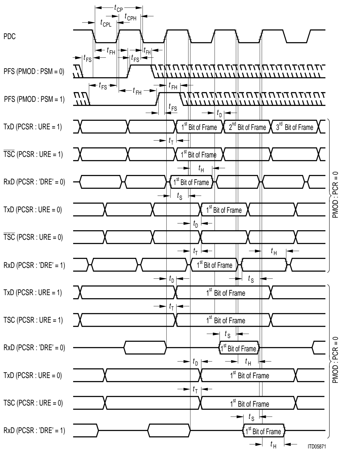
Figure 96 PCM-Interface Timing
