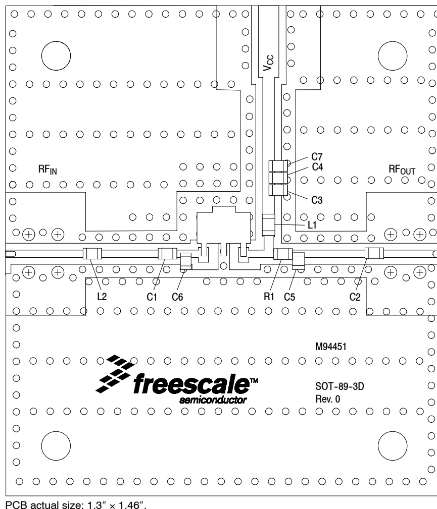
Figure 23. MMG30271BT1 Test Circuit Component Layout
