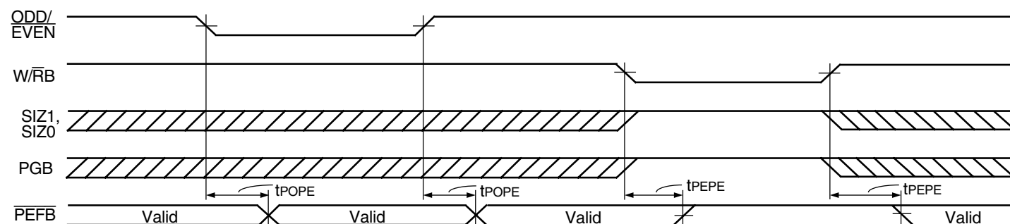
Figure 16. ODD/ \overline{EVEN} , W/ \overline{RA} , MBA, and PGA to \overline{PEFA} Timing
