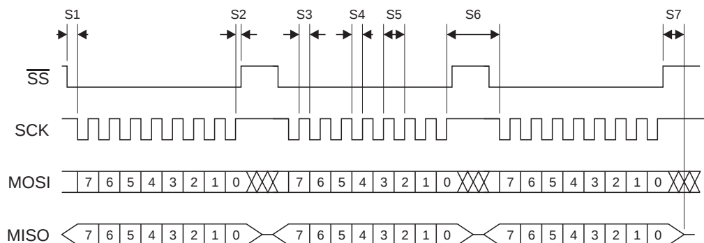
Figure 8-2. Data Byte Exchange – Timings
