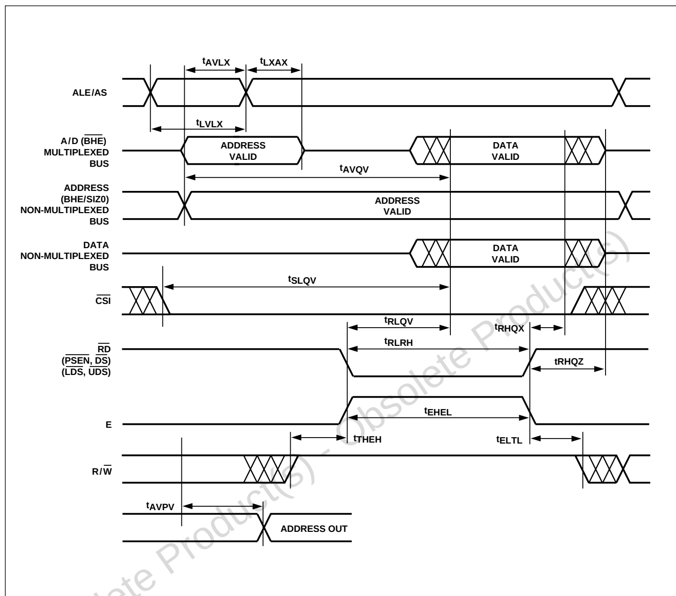
Figure 52. Read Timing
