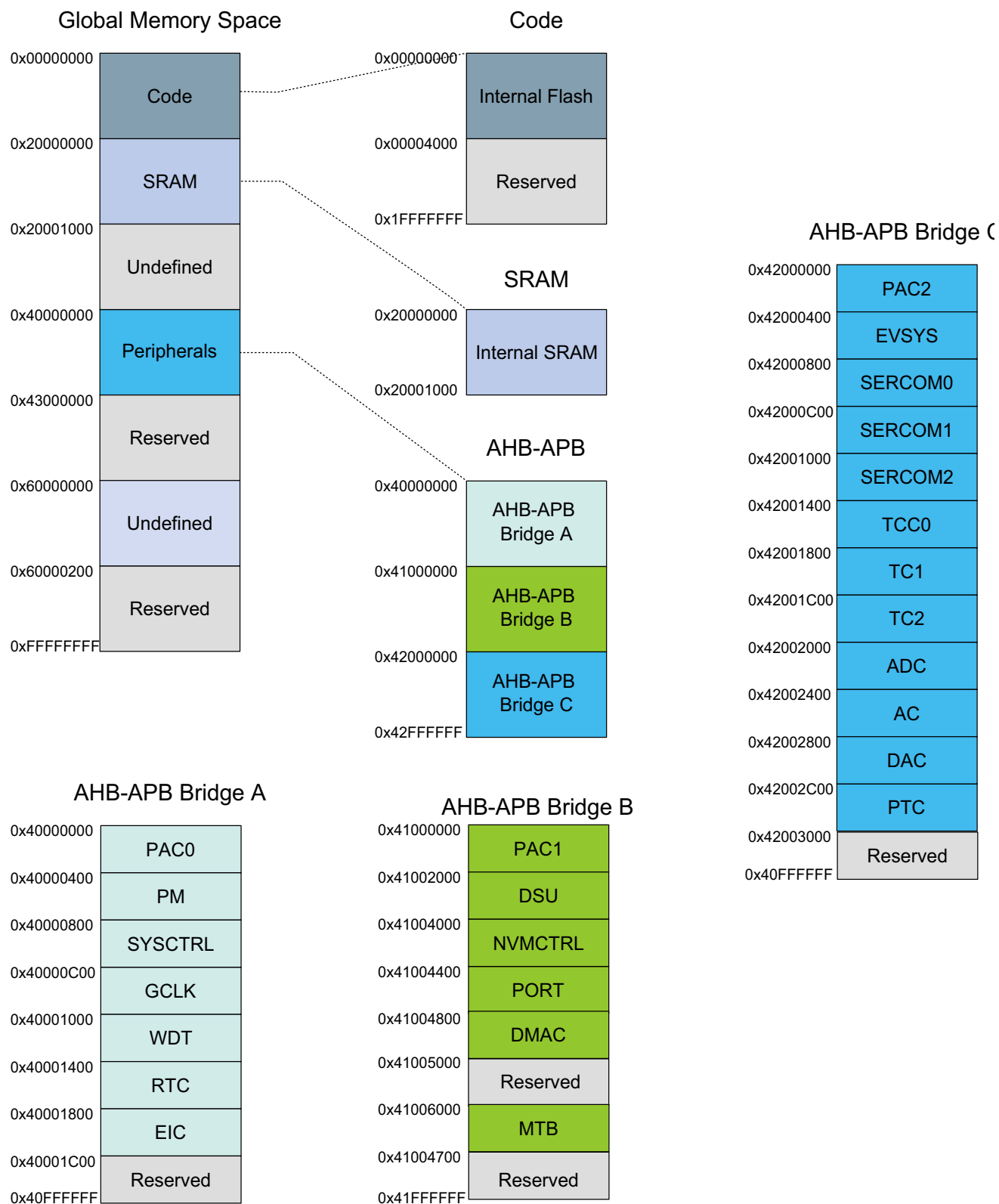
Figure 8-1. Atmel SAM D10 Product Mapping
