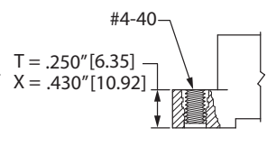
FLUSH MOUNTING WITH THREADED INSERT (T, X)
