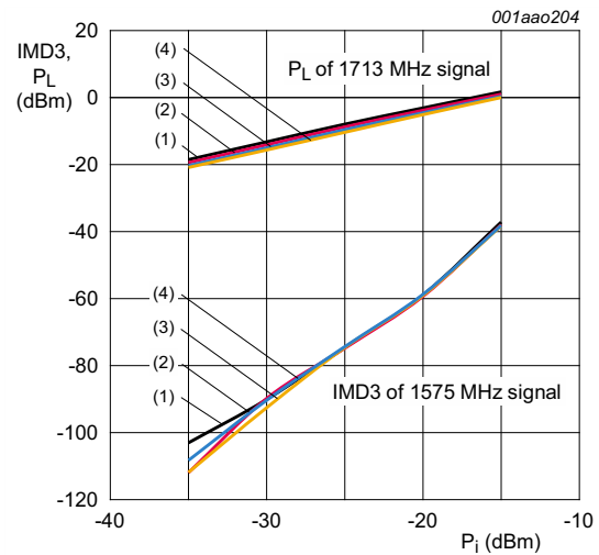
f = 1575 \text{ MHz}; f_1 = 1713 \text{ MHz}; f_2 = 1851 \text{ MHz}; V_{\text{CC}} = 1.8 \text{ V}. (1) T_{\text{amb}} = -40 \text{ }^{\circ}\text{C} (2) T_{\text{amb}} = +25 \text{ }^{\circ}\text{C} (3) T_{\text{amb}} = +85 \text{ }^{\circ}\text{C} (4) T_{\text{amb}} = +125 \text{ }^{\circ}\text{C}
