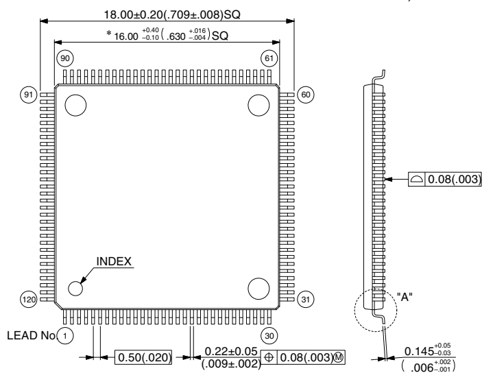
120-pin plastic LQFP (FPT-120P-M21)
