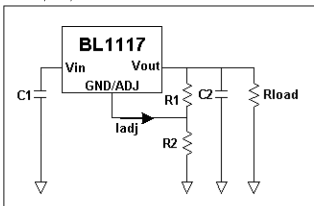
Chart 2. Application Circuit of BL1117 adjustable version
