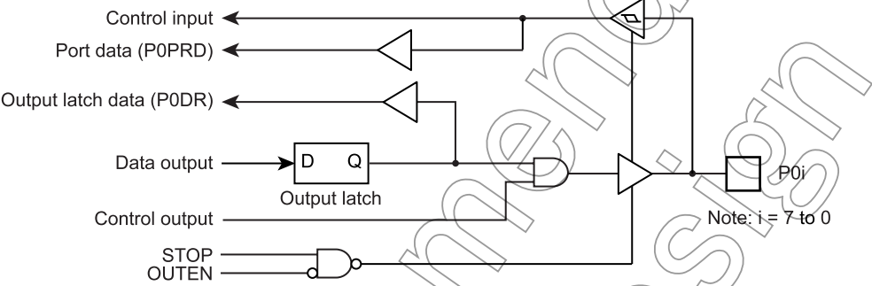
Figure 5-2 Port P0
