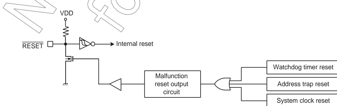
Figure 2-15 Reset Circuit
