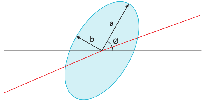
Figure 7. 3- and 5-step MacAdam ellipse illustration for Table 6.
