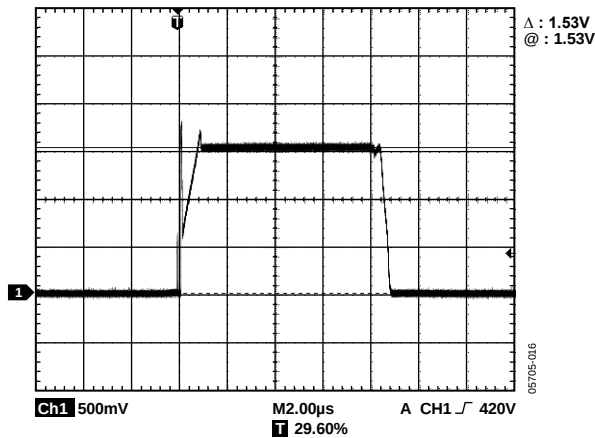
Figure 16. Power On/Off Response Time; V_P = 3.0V ; Input AC-Coupling Capacitors = 10pF ; C_{LPF} = Open
