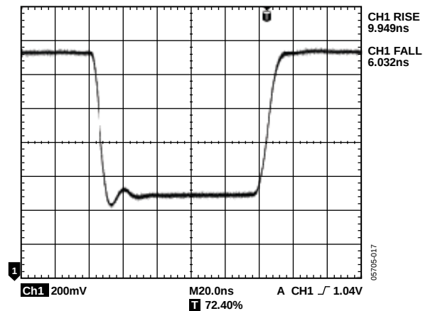
Figure 17. V_{OUT} Pulse Response Time; Pulsed RF Input 0.1GHz , -10dBm ; C_{LPF} = Open; R_{LOAD} = 150\Omega
