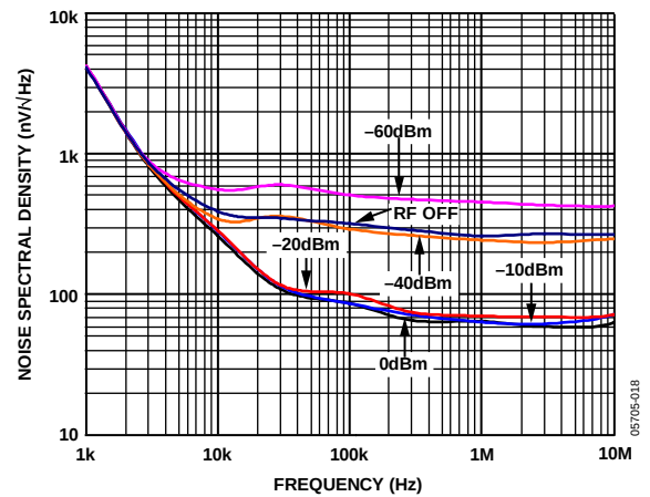
Figure 18. Noise Spectral Density of Output vs. Frequency; C_{LPF} = Open
