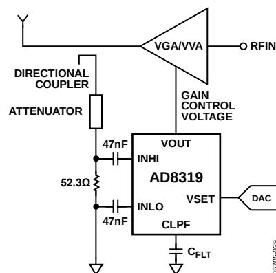
Figure 29. Controller Mode
