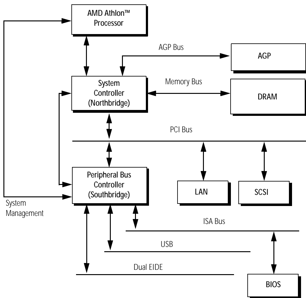
Figure 1. Typical AMD Athlon™ Processor Model 4 System Block Diagram
