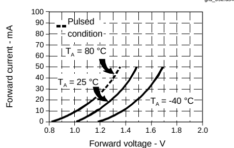
Fig. 1 IRED Forward Bias Characteristics
