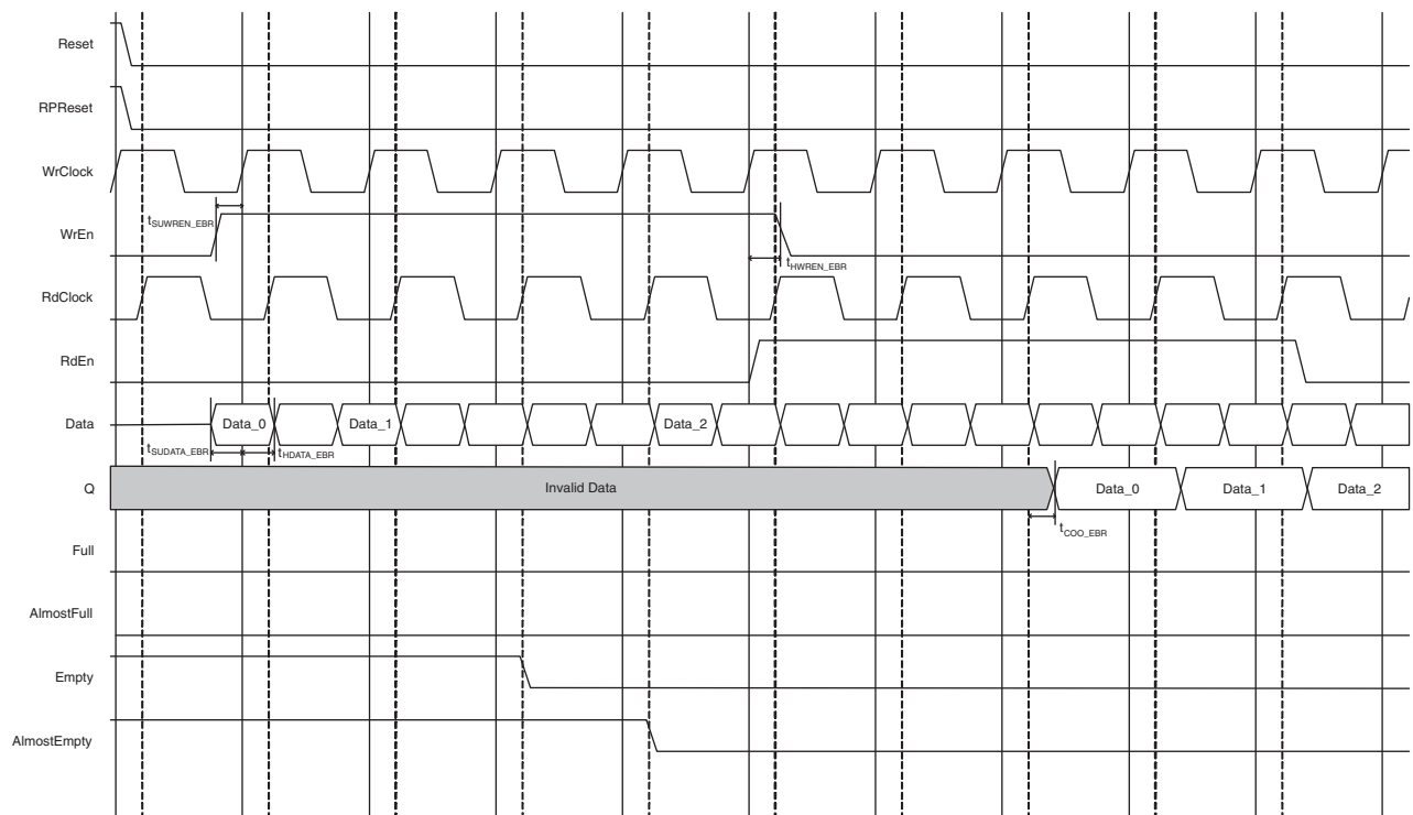
Figure 9-27. FIFO_DC with Output Registers (Pipelined)
