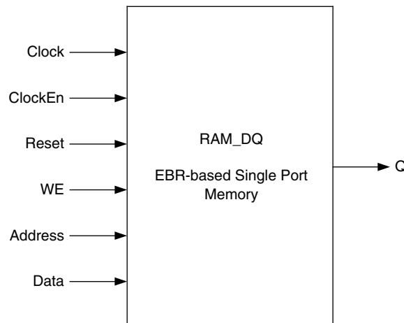
Figure 9-5. Single Port Memory Module Generated by IPexpress
