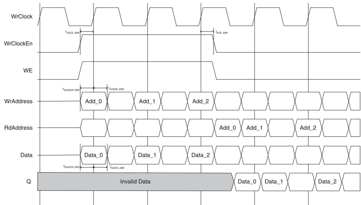
Figure 9-32. PFU-Based Distributed Dual Port RAM Timing Waveform – without Output Registers (Non-Pipelined)
