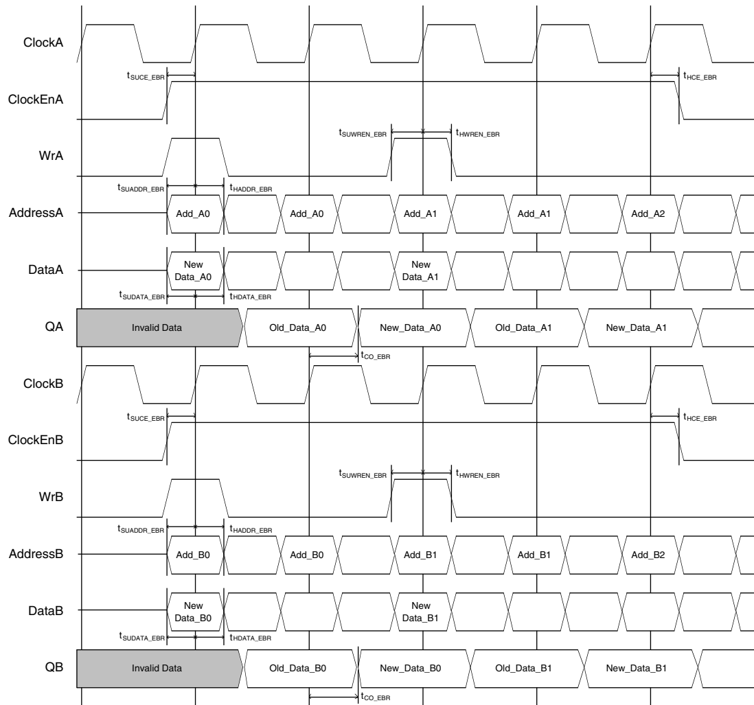
Figure 9-15. True Dual Port RAM Timing Waveform - READ BEFORE WRITE Mode, without Output Registers
