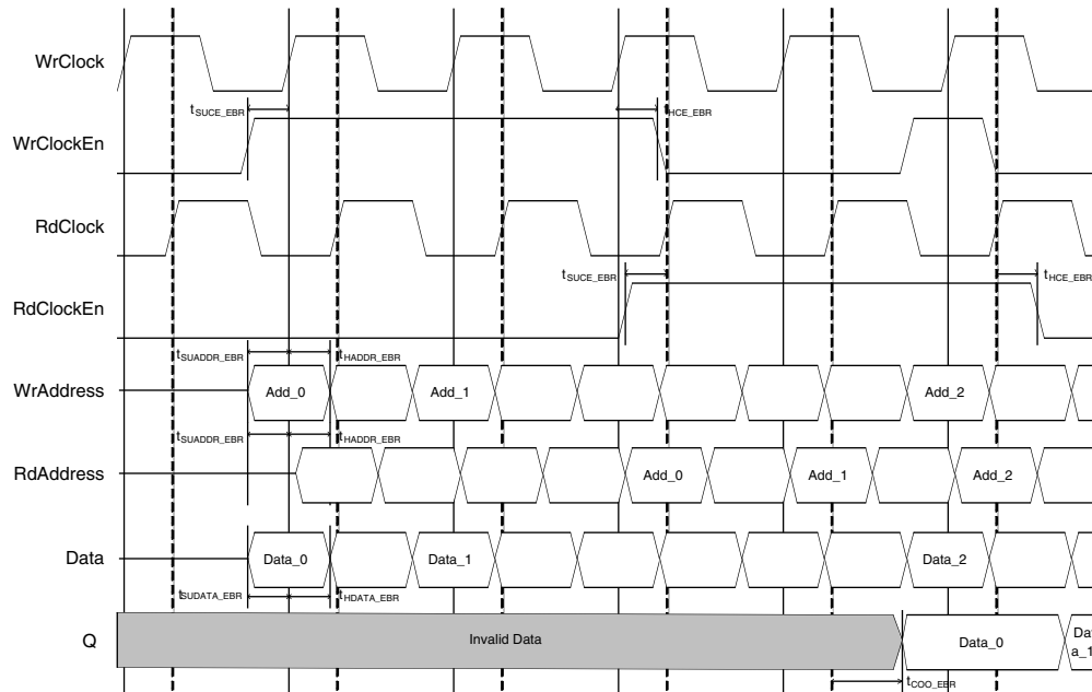
Figure 9-21. PSEUDO DUAL PORT RAM Timing Diagram – with Output Registers
