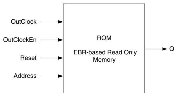
Figure 9-22. ROM – Read Only Memory Module Generated by IPexpress
