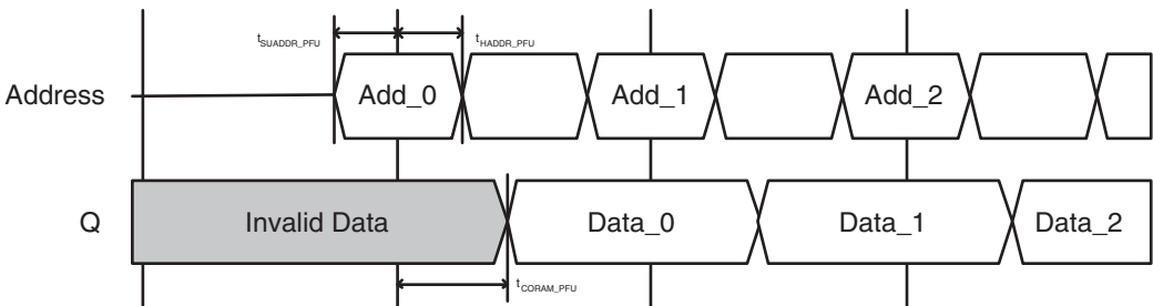
Figure 9-35. PFU-Based ROM Timing Waveform – Without Output Registers
