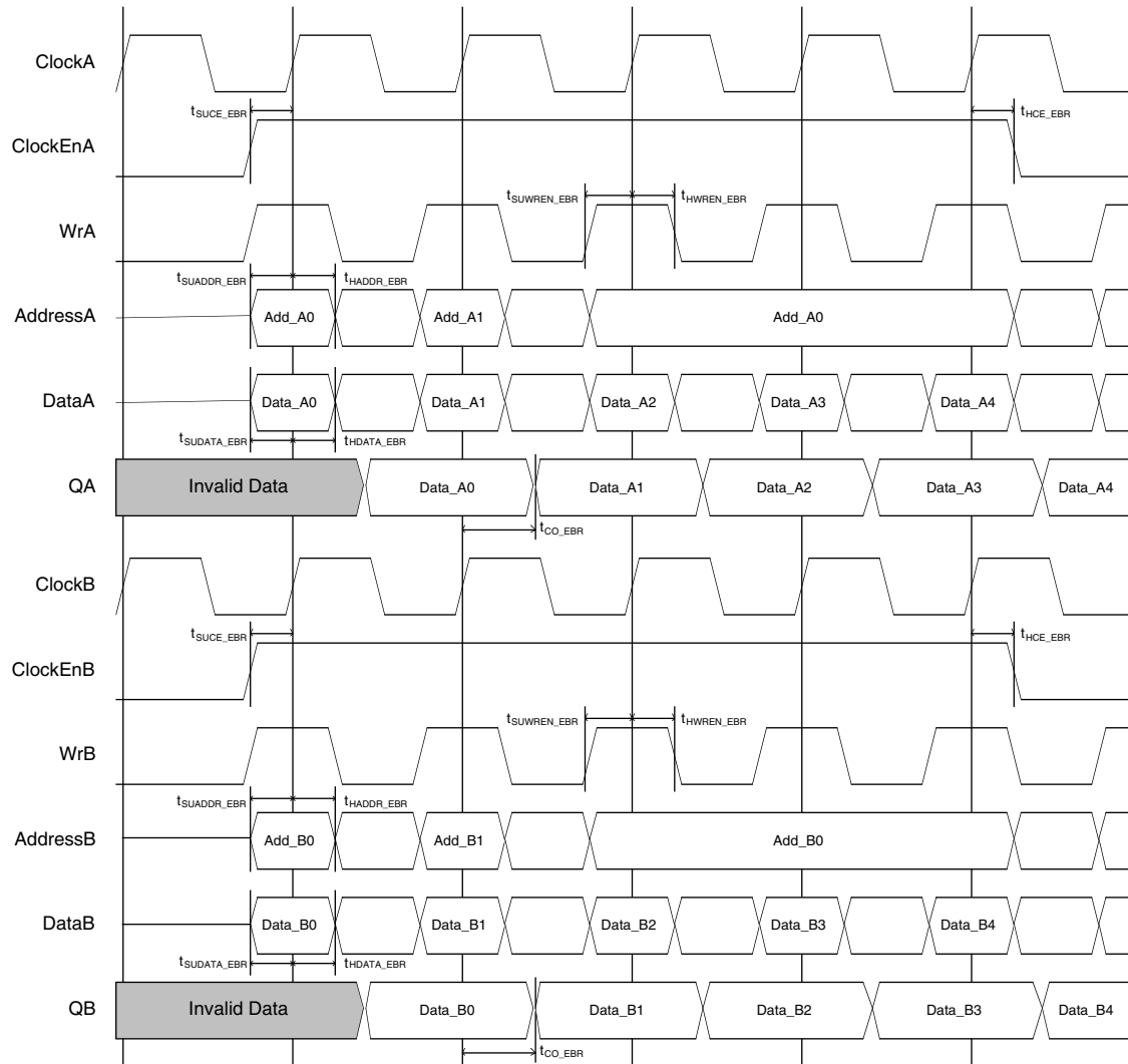
Figure 9-17. True Dual Port RAM Timing Waveform - WRITE THROUGH Mode, without Output Registers
