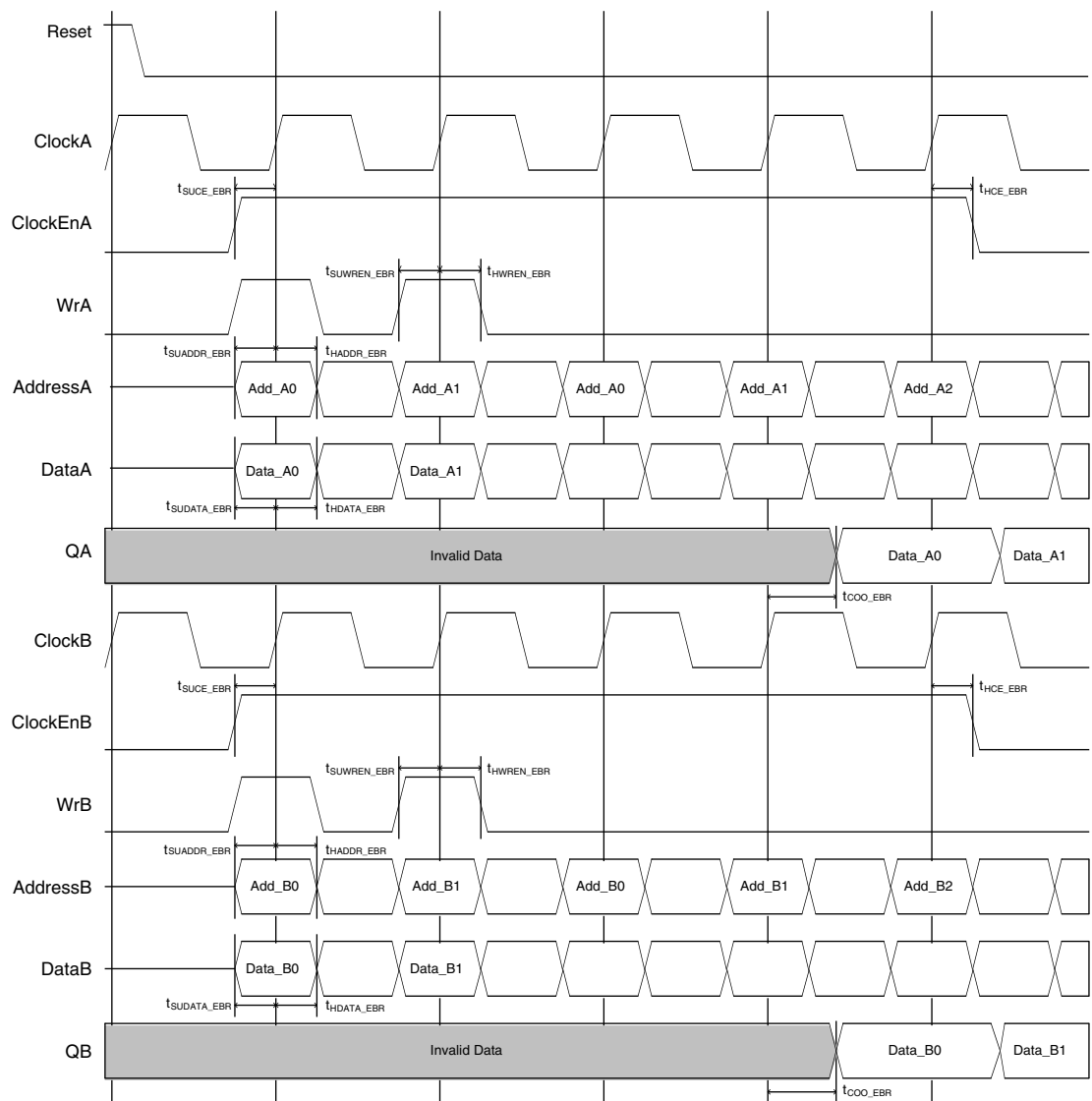
Figure 9-14. True Dual Port RAM Timing Waveform - NORMAL Mode with Output Register
