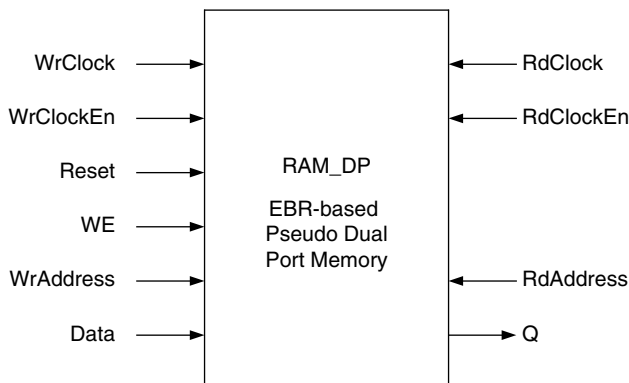
Figure 9-19. Pseudo Dual Port Memory Module Generated by IPexpress
