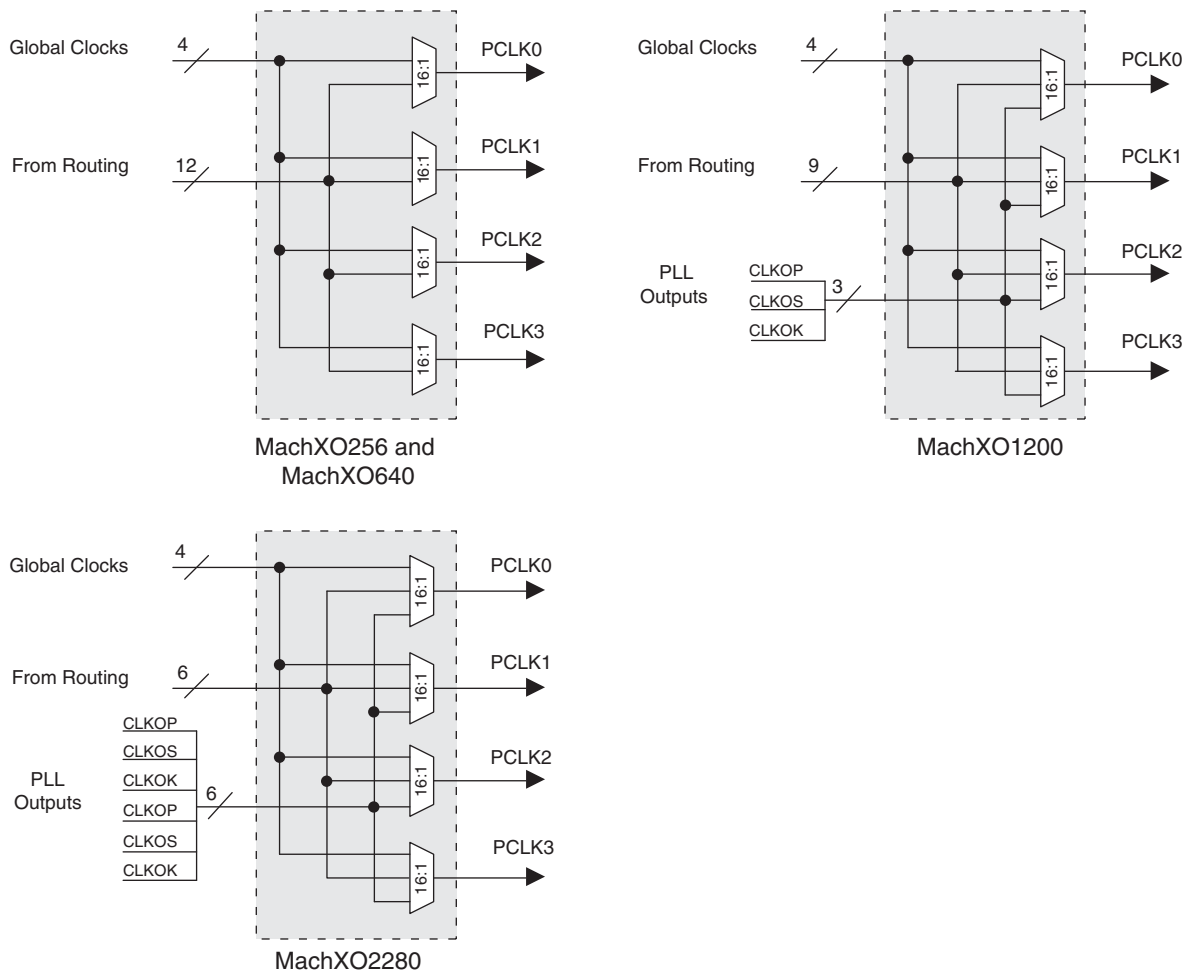
Figure 10-11. Primary Clock Net
