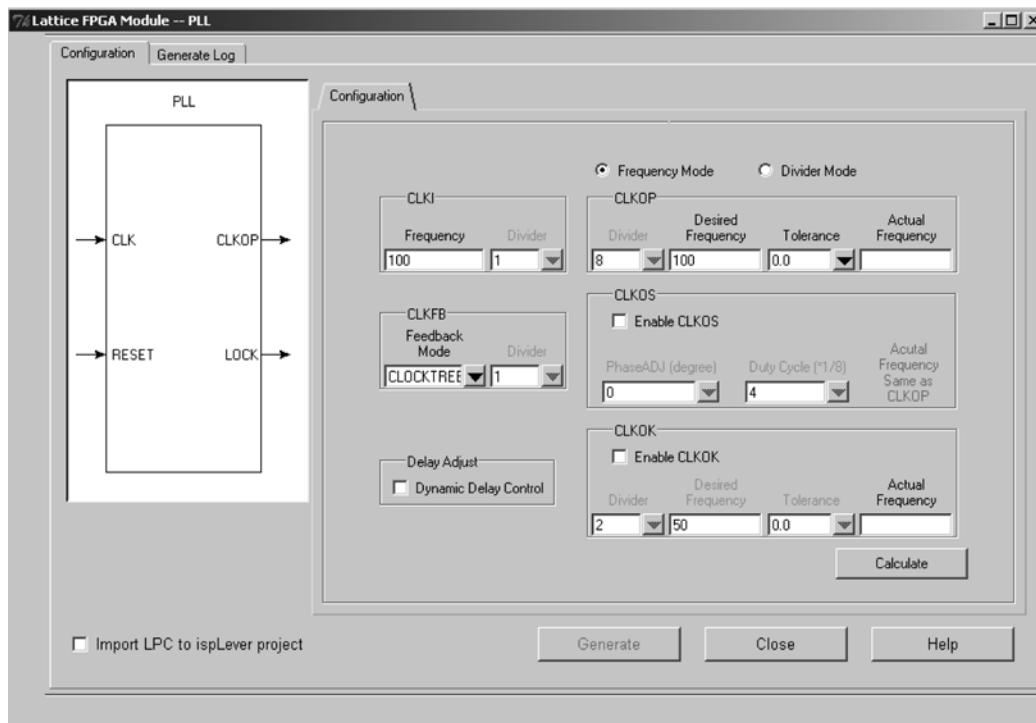
Figure 10-8. MachXO PLL Configuration Tab (Frequency Mode) Screen Capture
