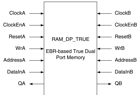
Figure 9-12. True Dual Port Memory Module generated by IPexpress
