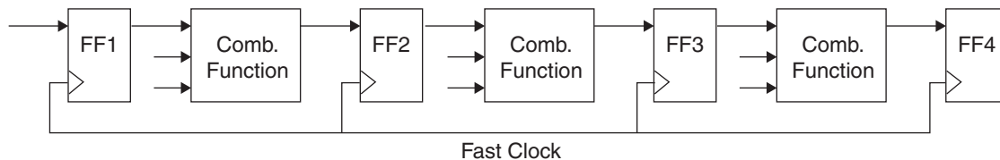
Figure 13-6. After Pipelining
