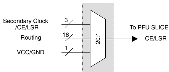
Figure 10-14. Control Switch Mux to Each PFU Slice
