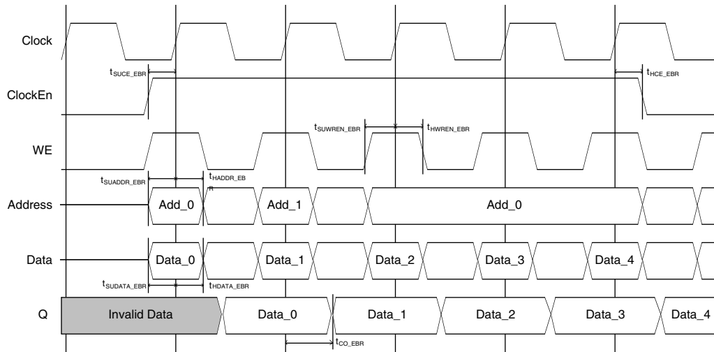
Figure 9-11. Single Port RAM Timing Waveform - WRITE THROUGH Mode, with Output Registers
