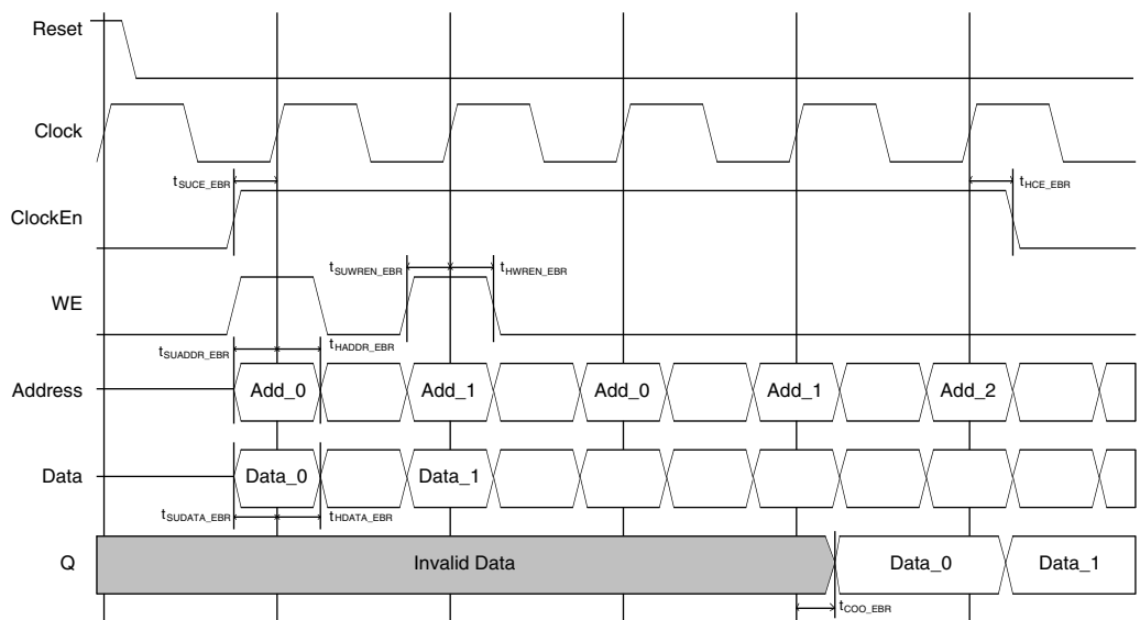
Figure 9-7. Single Port RAM Timing Waveform - NORMAL Mode, with Output Registers
