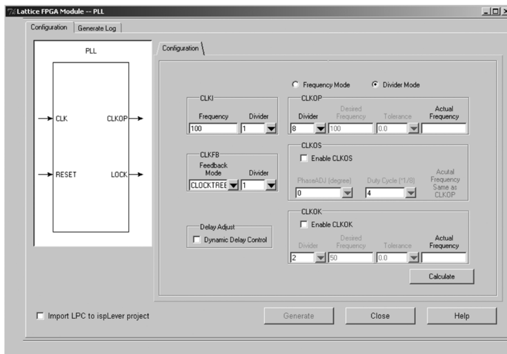
Figure 10-9. MachXO PLL Configuration Tab (Divider Mode)
