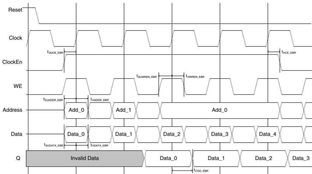
Figure 9-11. Single Port RAM Timing Waveform - WRITE THROUGH Mode, with Output Registers
