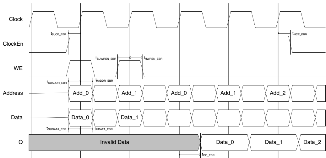
Figure 9-7. Single Port RAM Timing Waveform - NORMAL Mode, with Output Registers
