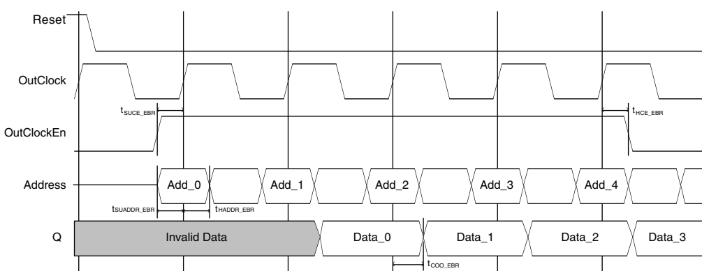
Figure 9-24. ROM Timing Waveform – with Output Registers
