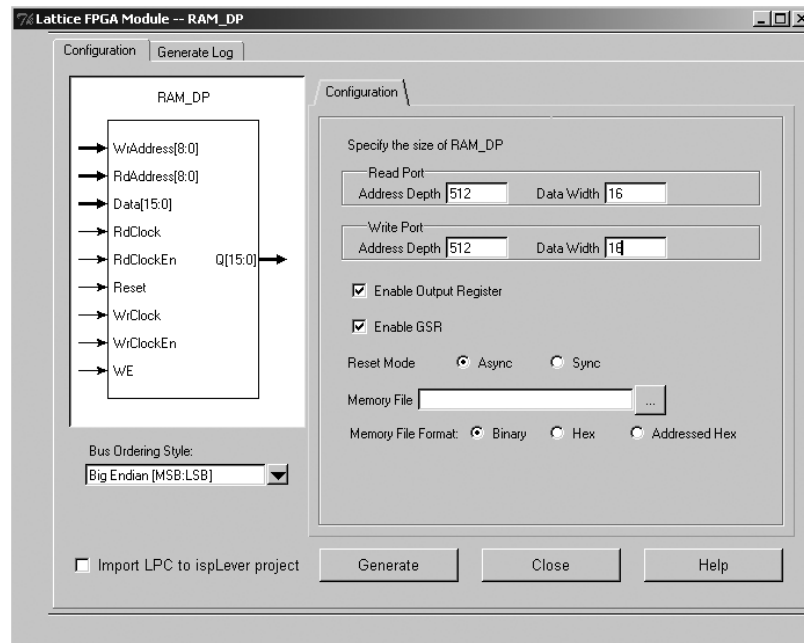
Figure 9-4. Example Generating Pseudo Dual Port RAM (RAM_DP) Module Customization
