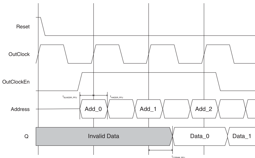
Figure 9-36. PFU-Based ROM Timing Waveform – with Output Registers
