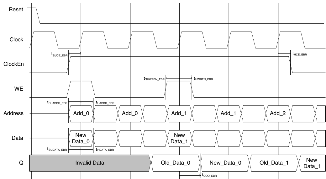
Figure 9-9. Single Port RAM Timing Waveform - READ BEFORE WRITE Mode, with Output Registers
