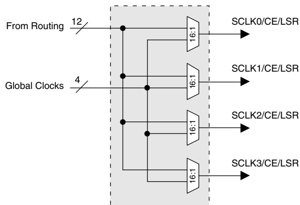
Figure 10-12. Secondary Clock/Control Net (All MachXO)
