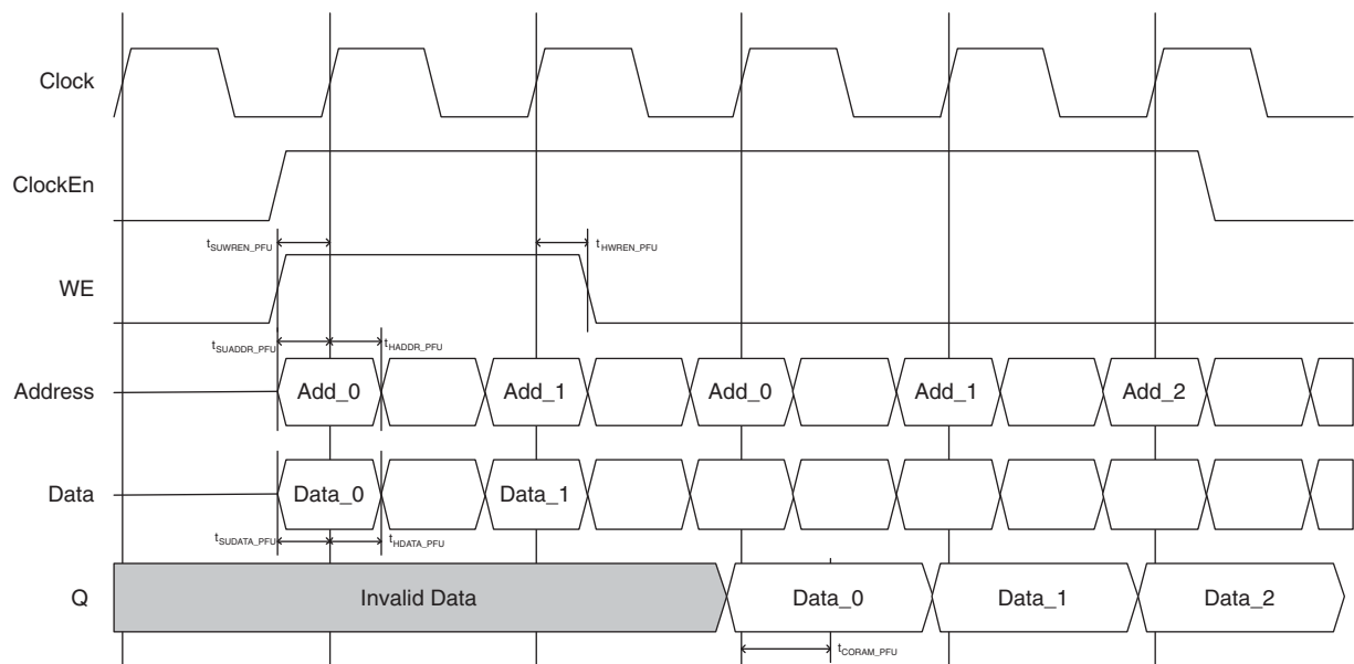
Figure 9-30. PFU-Based Distributed Single Port RAM Timing Waveform - With Output Registers
