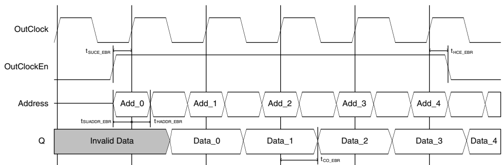
Figure 9-24. ROM Timing Waveform – with Output Registers
