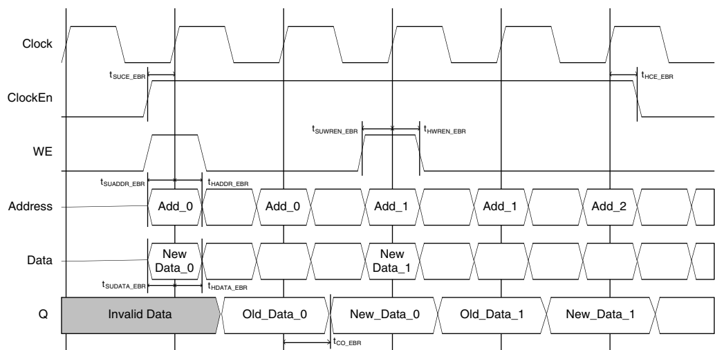
Figure 9-9. Single Port RAM Timing Waveform - READ BEFORE WRITE Mode, with Output Registers
