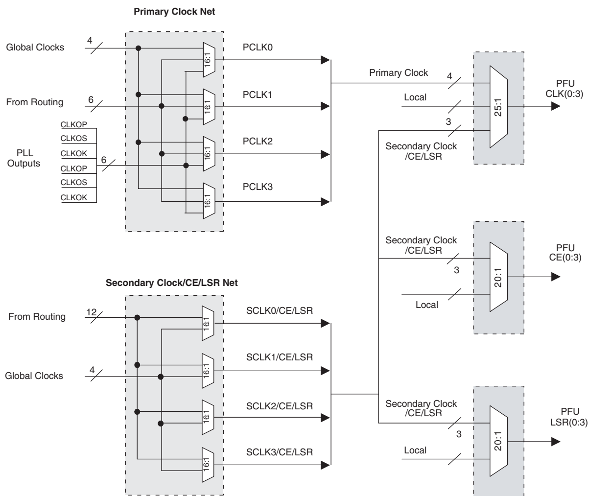
Figure 10-15. Primary Clock and Secondary Clock/CE/LSR Distribution
