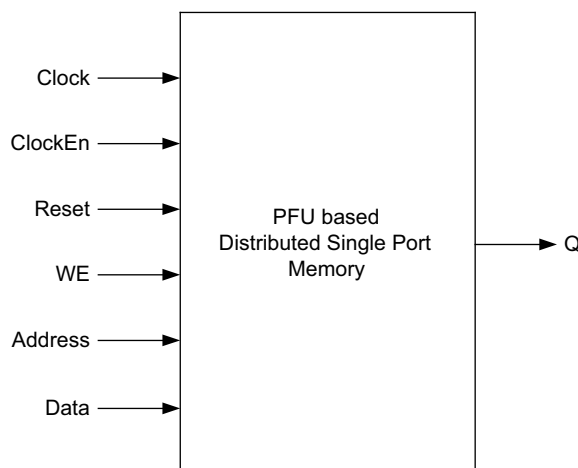
Figure 9-28. Distributed Single Port RAM Module Generated by IPexpress
