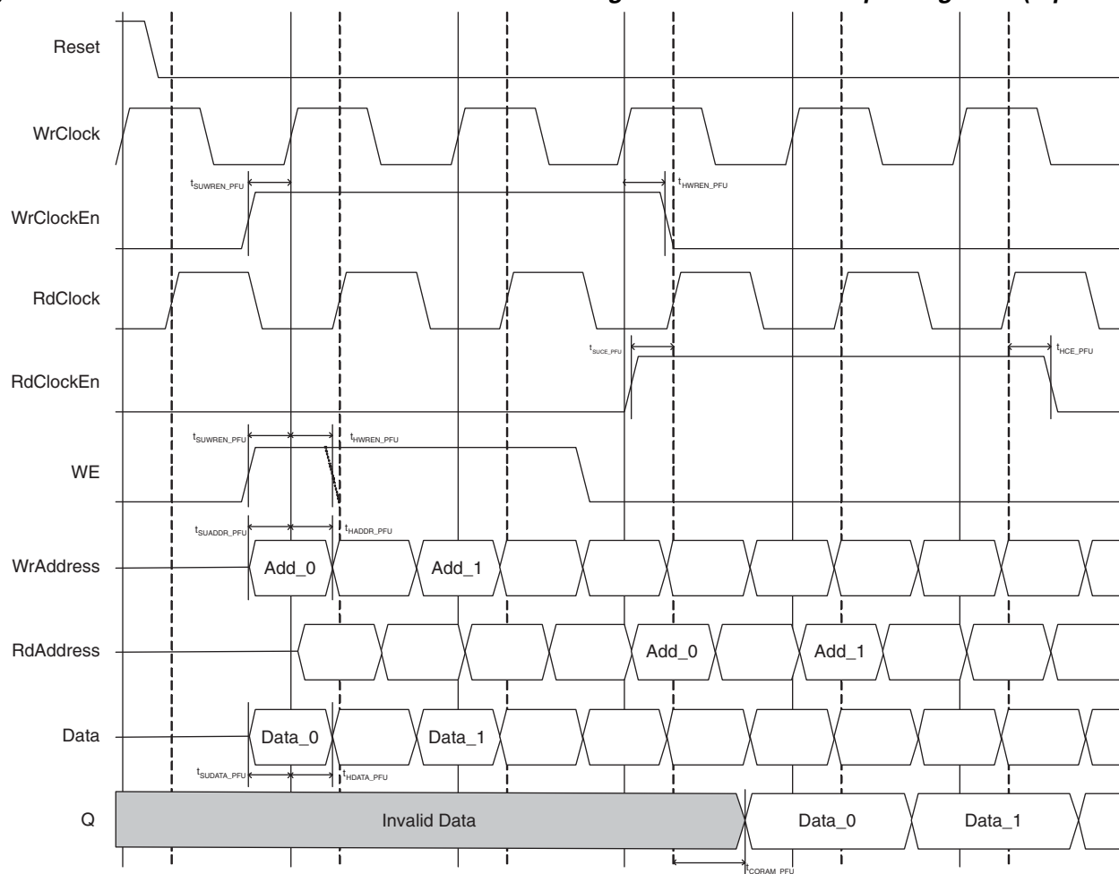
Figure 9-33. PFU-Based Distributed Dual Port RAM Timing Waveform – with Output Registers (Pipelined)
