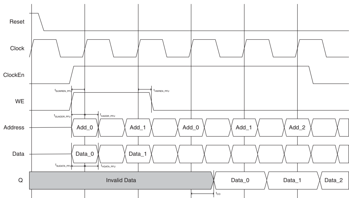
Figure 9-30. PFU-Based Distributed Single Port RAM Timing Waveform - With Output Registers
