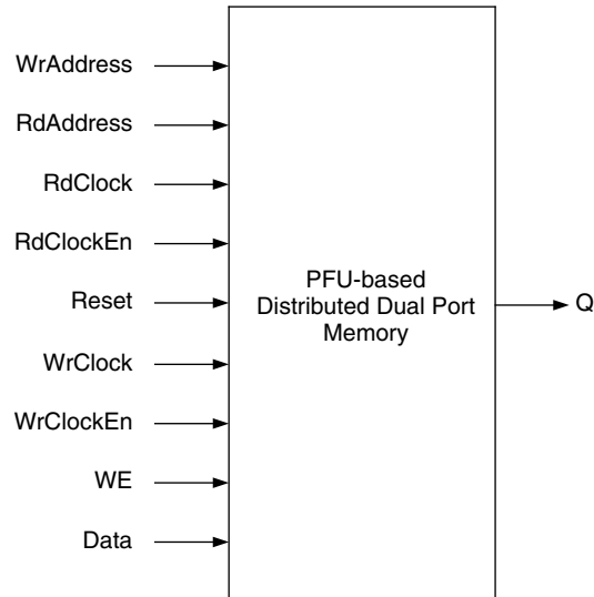
Figure 9-31. Distributed Dual Port RAM Module Generated by IPexpress
