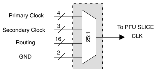
Figure 10-14. Control Switch Mux to Each PFU Slice
