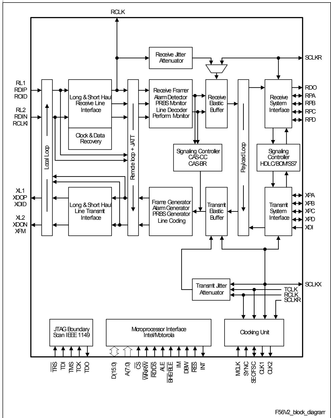
Figure 6 Block Diagram
