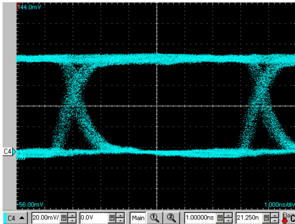
Figure 6. Eye Diagram
