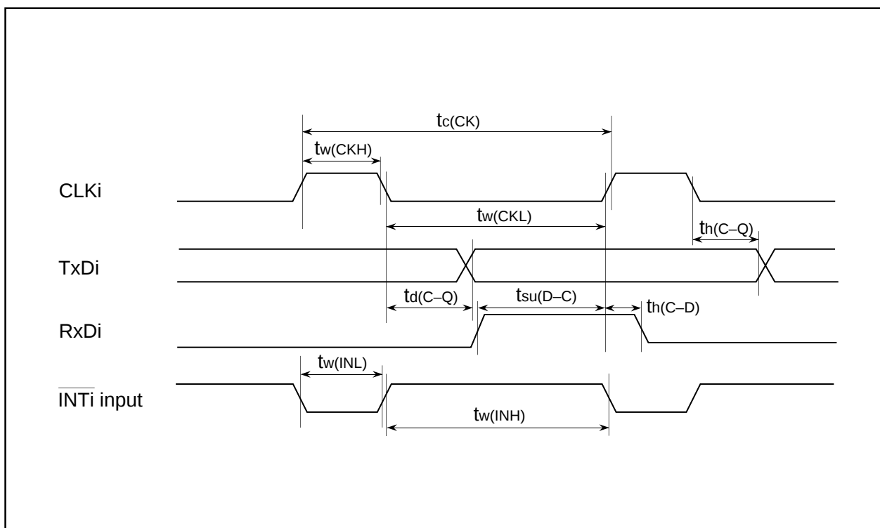
Figure 16.4. Timing Diagram (2)
