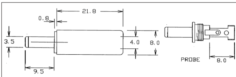
DCPP3 DC Line connector. Rated 12V / 5A. With 1.3mm dia. pin
