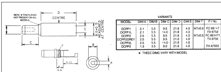
DCPP1 DC Line connector. Rated 12V / 5A. DCPP1 with 2.1mm dia. pin. DCPP2 with 2.5mm dia. pin.
